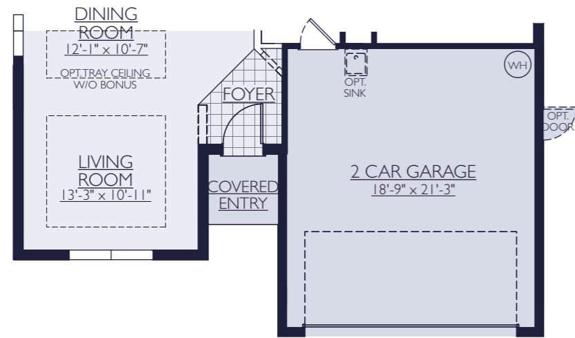
OPT 2' GARAGE EXTENSION
